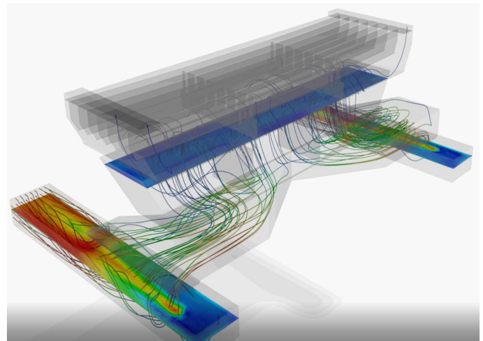
Output from Computational Fluid Dynamics (CFD) software
