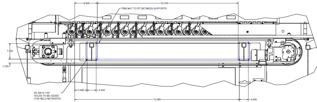
DETAIL E SCALE 1/6
